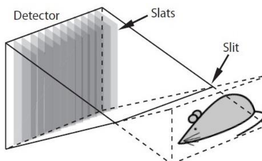
Figure 6. Illustration of FOVs with a slit-slat collimator that covers an entire mouse [52]
