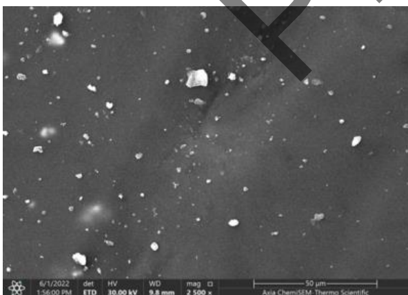
Figure 5. Scanning electron microscopy image of 5 wt. % TeO 2 specimens; 2500 magnification
